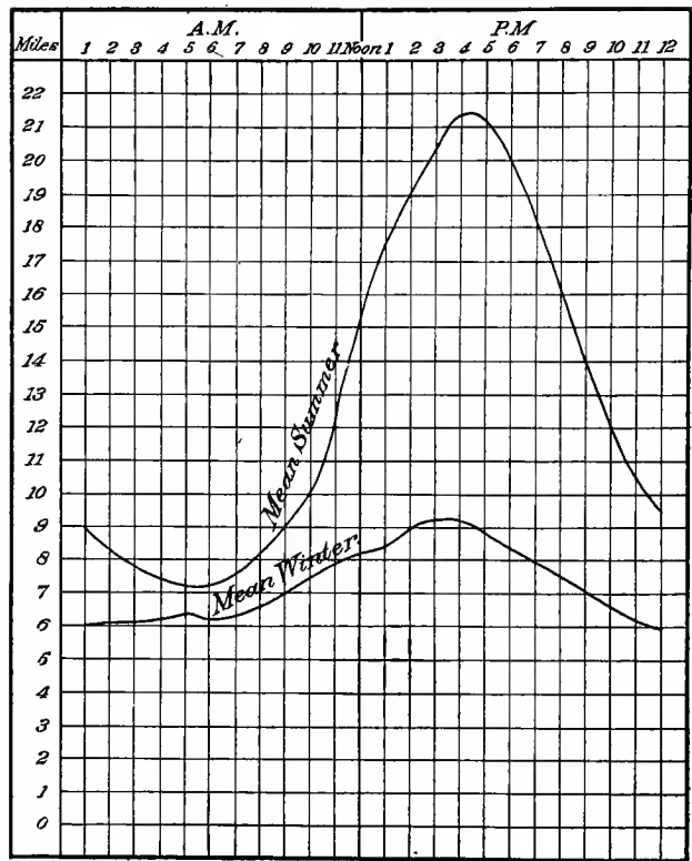
FIG. 7.—Hourly wind velocities at San Francisco.
